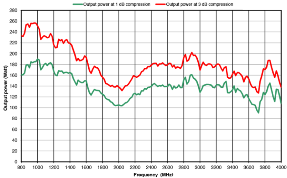
SW100 POWER AMPLIFIER 100W / 800 MHz - 4000 MHz
